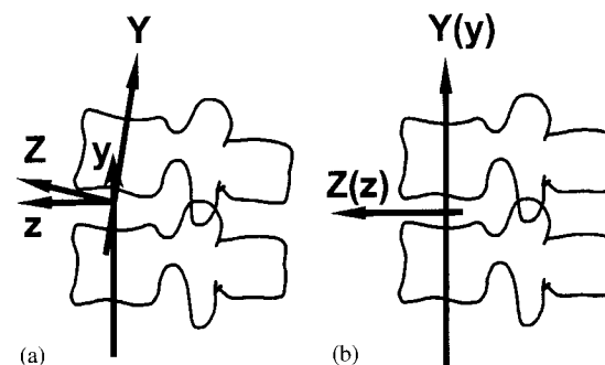
Fig. 5. Location of the common origin of axes: (a) the general case; (b) the specific case of Y and y being parallel. Note: the Y - and y -axis must be coplanar in the reference position of the two vertebrae.
