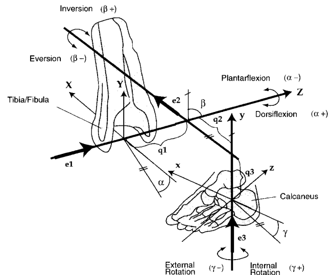
Fig. 2. Illustration of the JCS for the right ankle joint complex.
