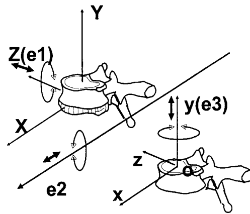
Fig. 4. Illustration of a proximal vertebral coordinate system ( XYZ ), a distal vertebral coordinate system ( xyz ), and the corresponding JCS.
