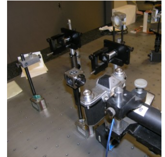
Figure 3: Interferometric method
