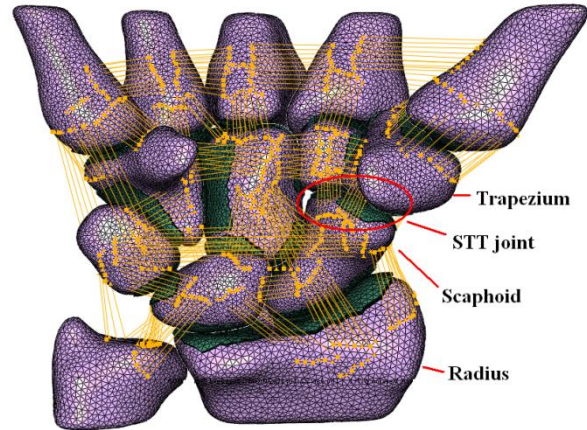
Figure 1: A finite element model of the wrist.
